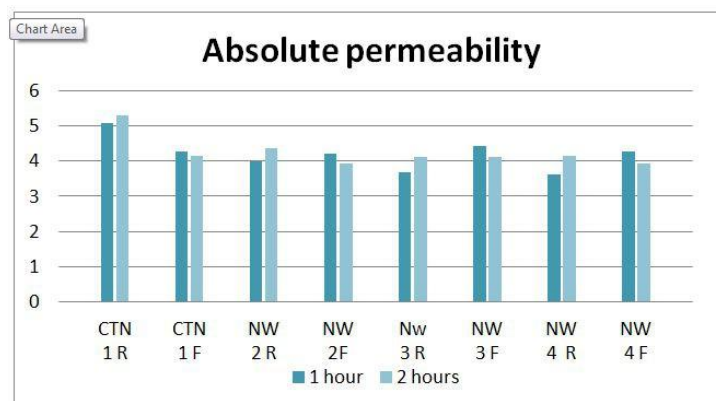
Figure 4. Histogram of absolute permeability depending on the type of material ( \frac{mmmm}{ccmm^2 \cdot h} ) Note: Meaning of the abbreviations CTN - cotton, NW - non woven
