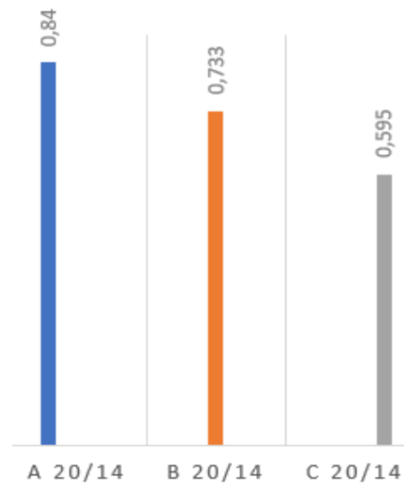
Figure 5: Absolute water vapour permeability for 4 hours ( \text{mg}\cdot\text{cm}^{-2}\cdot\text{h}^{-1} )
