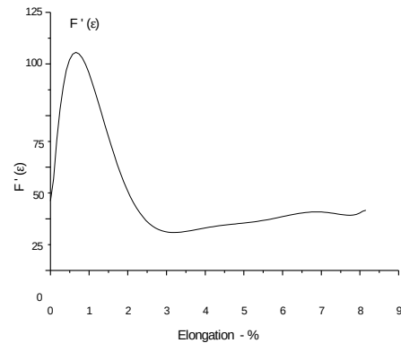
Figure 3: Dependence of F'(\epsilon) to the yield point
