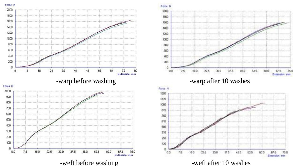
Figure 5. Breaking force before and after washing on sample 2 in the direction of the warp and weft
