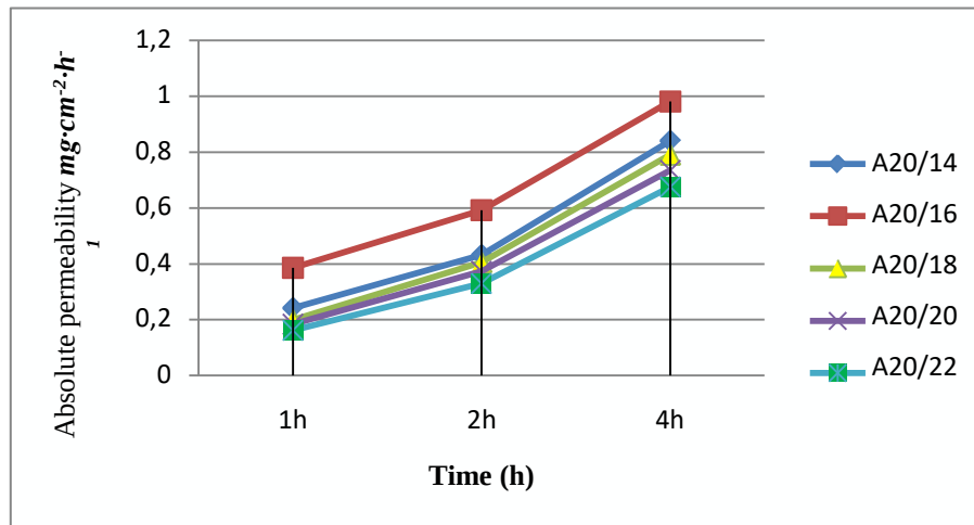
Figure 2: Absolute water vapour permeability for fabric A in plain weave ( \text{mg}\cdot\text{cm}^{-2}\cdot\text{h}^{-1} )
