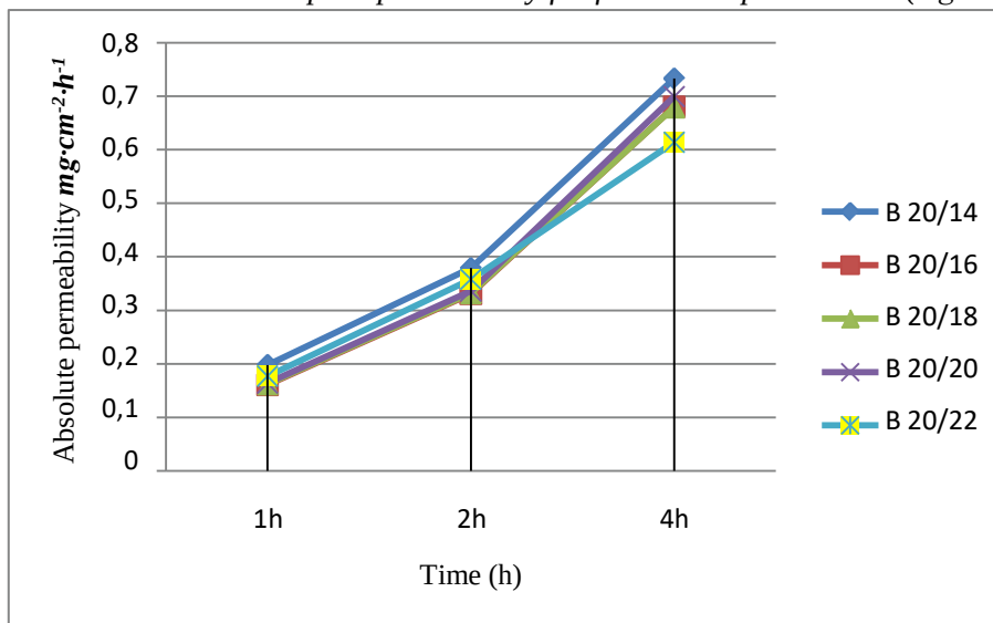
Figure 3: Absolute water vapour permeability for fabric B in twill 3:1 interweave ( \text{mg}\cdot\text{cm}^{-2}\cdot\text{h}^{-1} )
