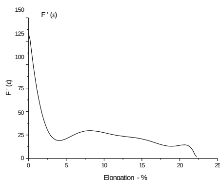
Figure 6: Dependence of F'(\epsilon) to break
