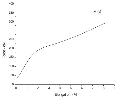
Figure 2: Dependence of F(\epsilon) to the yield point
