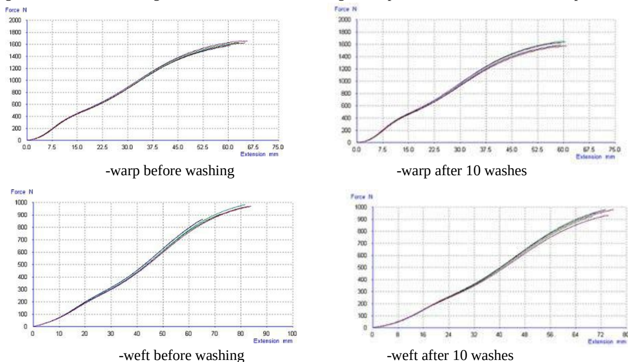
Figure 4. Breaking force before and after washing on sample 1 in the direction of the warp and weft Figure 5 shows the breaking force in the direction of the warp and weft before and after washing in sample 2.
