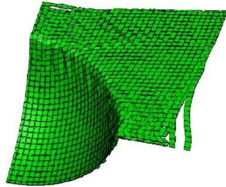
(b) A quarter of the deformed knitwear
