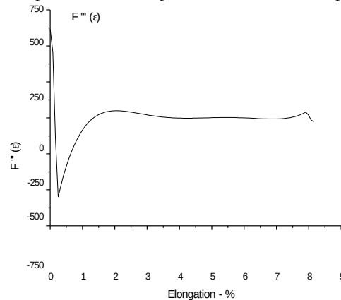
Figure 5: Dependence of F'''(\epsilon) to the yield point
