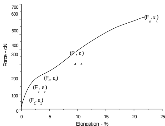
Figure 1 Curve F(\epsilon) of multifilament polyester yarn
