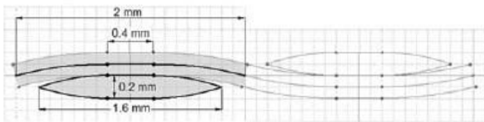
(a) unit cell and yarn models
