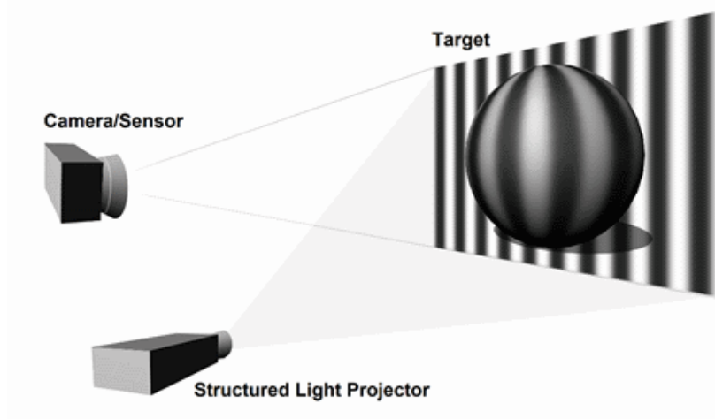
Figure 4: Projection of white light patterns
