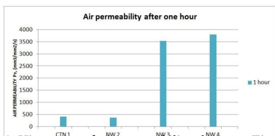
Figure 6. Histogram of air permeability change for each sample after one hour
