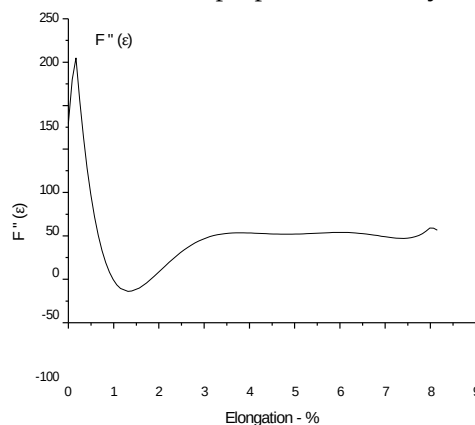
Figure 4: Dependence of F''(\epsilon) to the yield point
