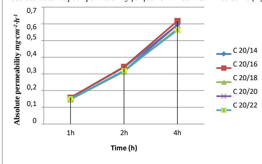
Figure 4: Absolute water vapour permeability for fabric C in twill 4:1 interweave ( \text{mg}\cdot\text{cm}^{-2}\cdot\text{h}^{-1} )
