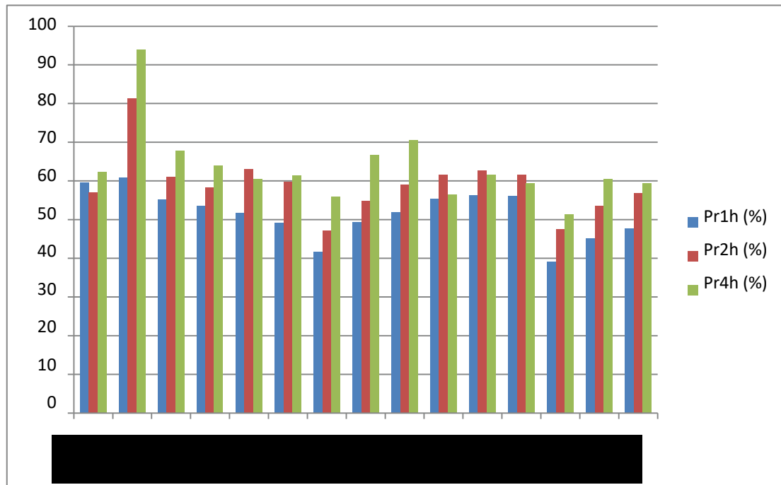
Figure 6: Histogram of the changes in relative permeability depending on the type of intertwine (%)
