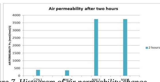
Figure 7. Histogram of air permeability change for each sample after two hours
